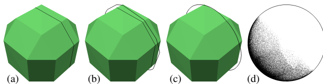
Figure 2: Silhouette projection from the base mesh to the implicit surface, silhouette subdivision, and final result with stippling.
