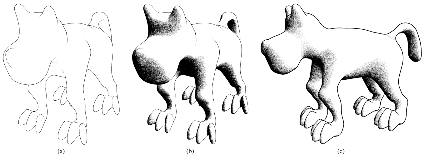
Figure 7: Complex model rendered using our technique with silhouettes and suggestive contours (a) as well as with additional stippling (b). A different view of the model with silhouette lines, suggestive contours, and stippling is shown in (c).
