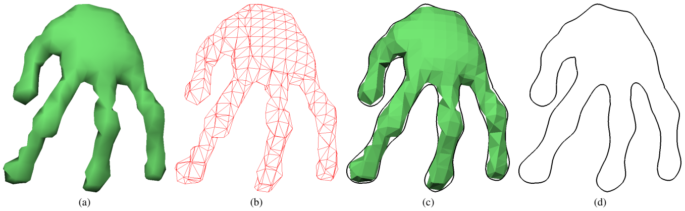
Figure 5: Implicit surface with relatively fine details: (a) Gouraud-shaded and (b) wireframe images of the implicit surface's low-res base mesh, (c) base mesh with silhouette, and (d) silhouette only.
