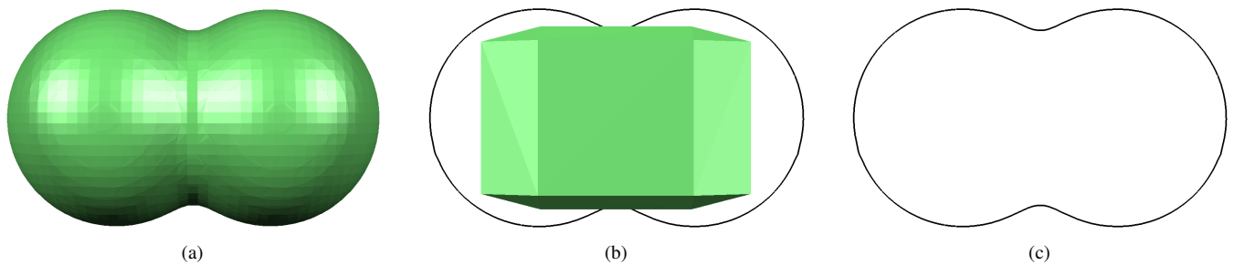
Figure 4: An extreme example of our silhouette refinement algorithm. The base mesh in (b) is a very low-resolution polygonization of the shape in (a). However, the silhouette (c) from this low-resolution base mesh, once projected and refined, is still quite accurate.
