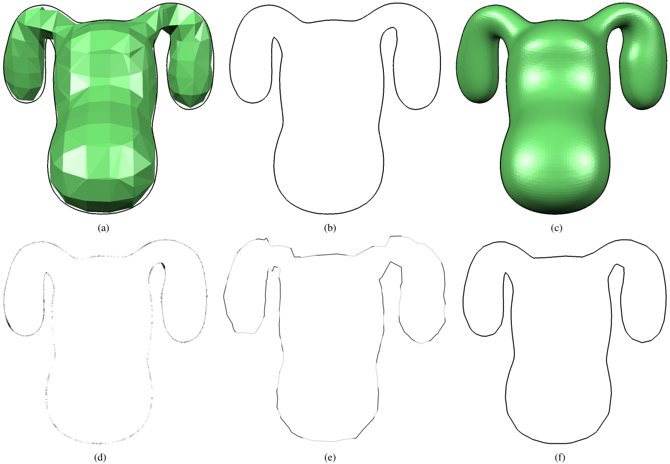
Figure 3: Silhouette example on a low-resolution mesh of a simple implicit surface. A low-resolution base mesh is shown in (a), the smooth silhouette extracted using our method is shown in (b). The silhouette is nearly identical to the high-resolution silhouette in (c), as shown in the difference image (d). For comparison, the low-resolution mesh silhouette is shown in (e), and the low-resolution silhouette after projection but before subdivision is shown in (f). The projection step alone clearly provides a significant improvement in silhouette quality, however subdivision is necessary to impart a real sense of smoothness (b).
