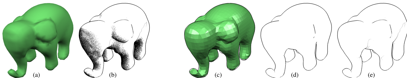
Figure 1: An implicit surface model visualized using a smooth-shaded triangle mesh (a) and a pen-and-ink drawing (b). The generated silhouettes (d) are much smoother than base mesh (c) and render at interactive rates. Suggestive contours (e) add important additional detail.
